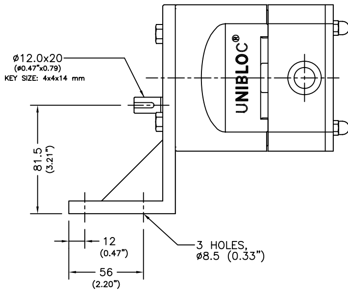
HORIZONTAL THROUGH-PUT
